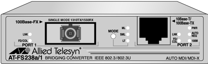
Figure 1 AT-FS238a/x Series Front Panel (AT-FS238a/1 Model)
